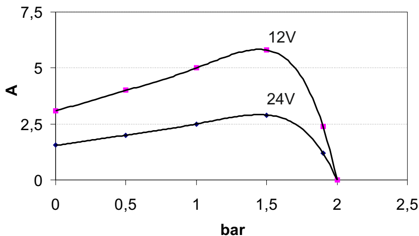
AMPERE-DRAW DIAGRAM
